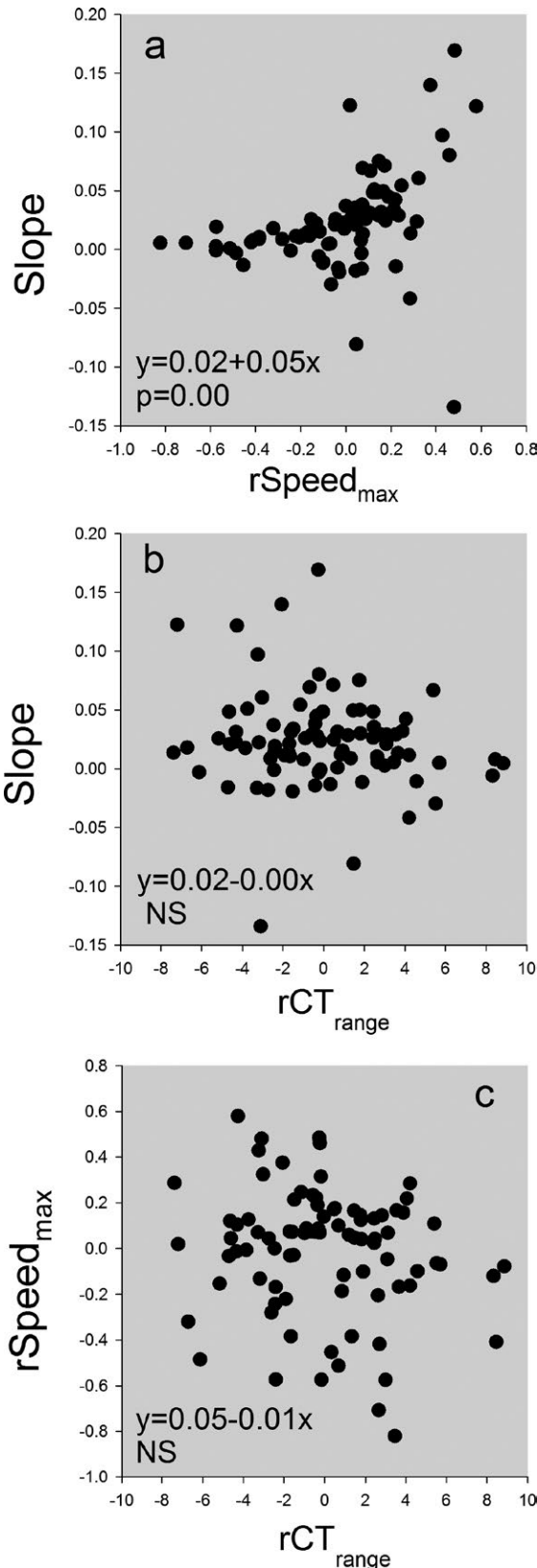
FIG. 4. Testing for interspecific tradeoffs among the three parameters describing ant thermal performance. Slope is the thermal sensitivity of speed, (i.e., the slope of speed vs. temperature from 20–35°C); rSpeed_{max} is the mass corrected speed (the residual of body mass versus maximum speed, see Fig. 3); rCT_{range} is mass corrected thermal range (i.e., the residual of body mass versus CT_{max}-CT_{min} ). RMA regression results are embedded.
