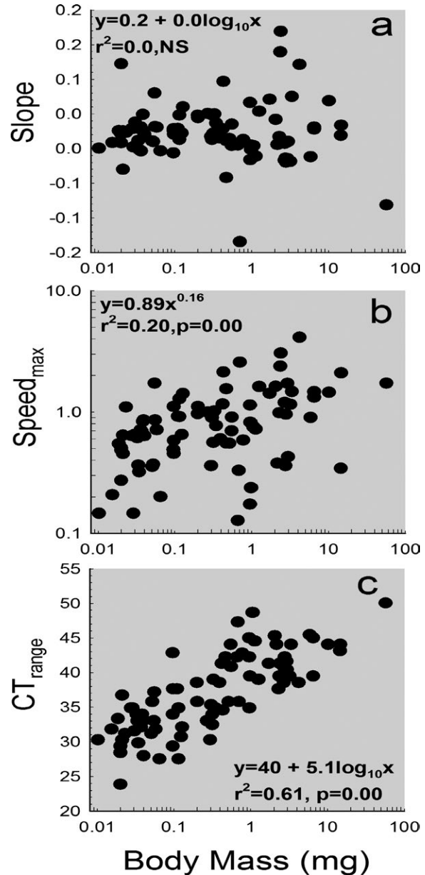
FIG. 3. Three parameters from 87 ant thermal performance curves scaled to body mass. (a) Slope represents the LSM regression estimate of the change in an ant's speed from 20 to 35°C. (b) Speed_{max} ( cm^{-s} ) is the maximum speed recorded for the species. (c) CT_{range} ( ^{\circ}C ) is the span of surface temperatures at which ants were active.
