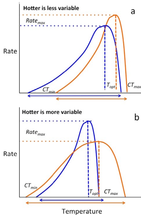
FIG. 1. Predicted shapes of Thermal Performance Curves (TPCs) under Thermal Adaptation when temperature mean and variance are positively or negatively correlated. Horizontal arrows represent the range of environmental temperature experienced by individuals in a pair of habitats, orange and blue. (a) Where warmer environments are less variable (e.g., along the latitudinal gradient), warmer environments generate temperature specialists with higher maximum performance. (b) Where warmer environments are more variable, warmer environments favor temperature generalists with lower maximum performance. CT_{min} and CT_{max} are the low and high temperatures at which performance ceases, Rate_{max} is the peak performance rate, and T_{opt} is the temperature at which Rate_{max} occurs.
