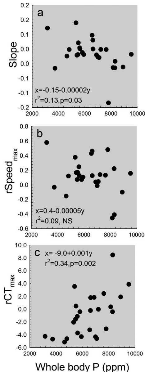
FIG. 6. Tests of the Phosphorus-Tolerance hypothesis for 26 Panama ant species. The concentration of P in ant tissue is related to (a) the thermal sensitivity of speed, (i.e., the slope of speed vs. temperature from 20–35°C) (b) r\text{Speed}_{\text{max}} , the mass corrected speed (i.e., the residual of the maximum speed versus temperature, see Fig. 3); (c) r\text{CT}_{\text{max}} , the mass corrected thermal maximum (i.e., the residual of body mass versus \text{CT}_{\text{max}} ).
