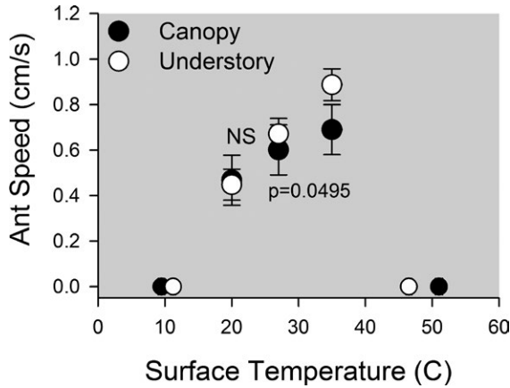
FIG. 2. Thermal performance curves of ant species nesting in the canopy and understory. (a) the LSMeans average speed ( \pm SE) at 20, 27 and 35°C, bounded by the average CT_{min} and CT_{max} (SE's too small to be visible). P values reflect Kruskal-Wallis comparisons of average rates of change for speed from 20 to 27°C, and from 27 to 35°C.
